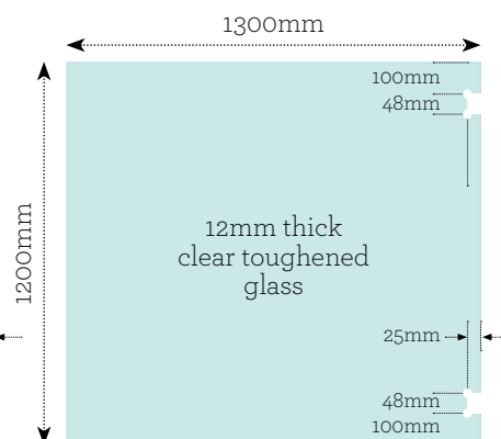
Order Code: SCE1312HP PH Glass weight: 46.8kg
