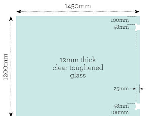
Order Code: SCE14512HP PH Glass weight: 52.2kg
