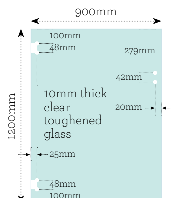
Order Code: SCE0912GP PH Glass weight: 28kg
