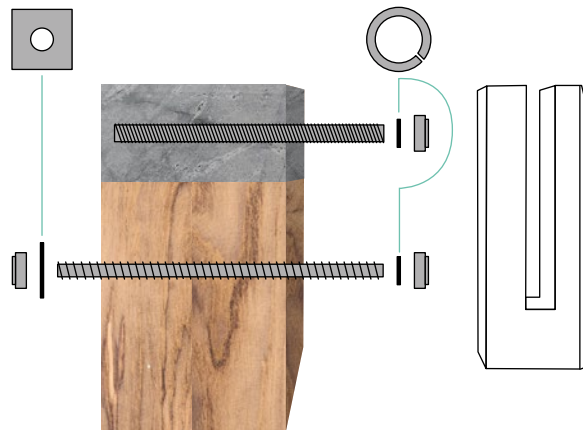
Backing Washer
